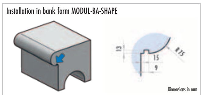
Installation in bank form MODUL-BA-SIZE
