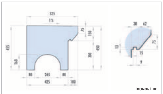
Bench seats in parallel arrangement (MODUL-ROOM-R ...)
